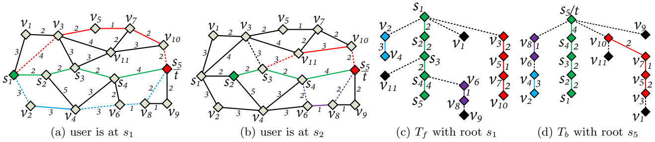
Figure 2: A sample road network where user's path P = \langle s_1, s_2, \dots, s_5 \rangle . Top-3 plateaus when user is at s_1 are pl(s_1, s_5) , pl(v_3, v_{10}) and pl(v_2, v_4) .
